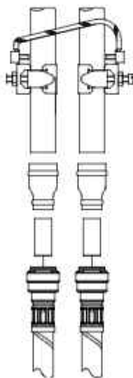
Figure 11 Earth continuity connections
