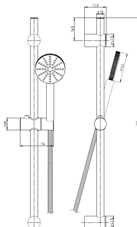
Dimensions (measurements in mm)
